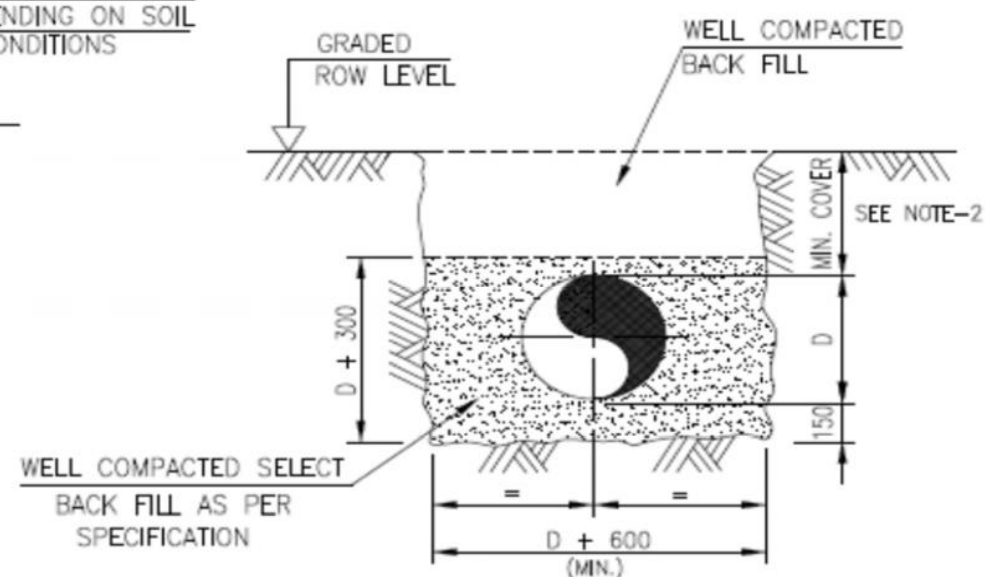
TRENCH IN CONSOLIDATED ROCK TYPICAL SECTION
