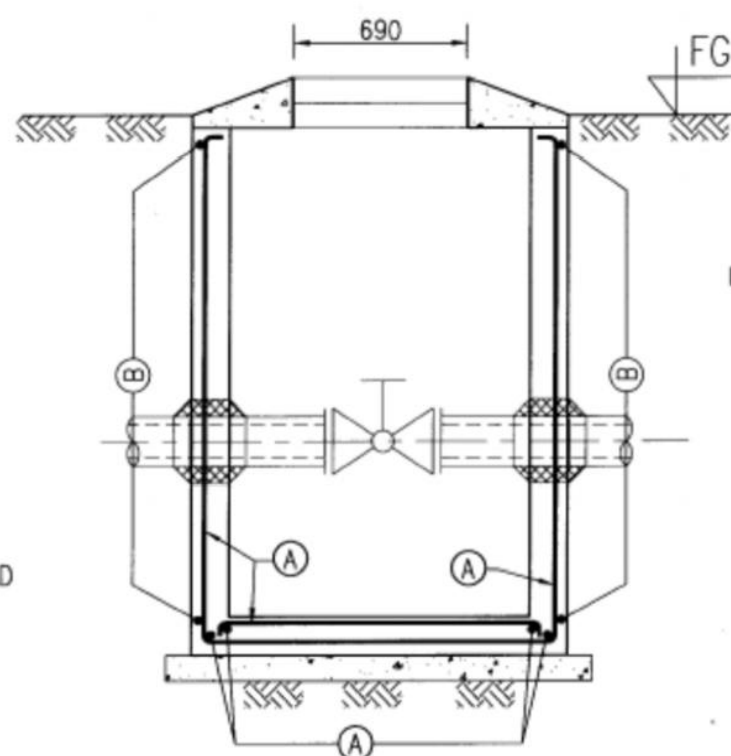
SECTION B-B
