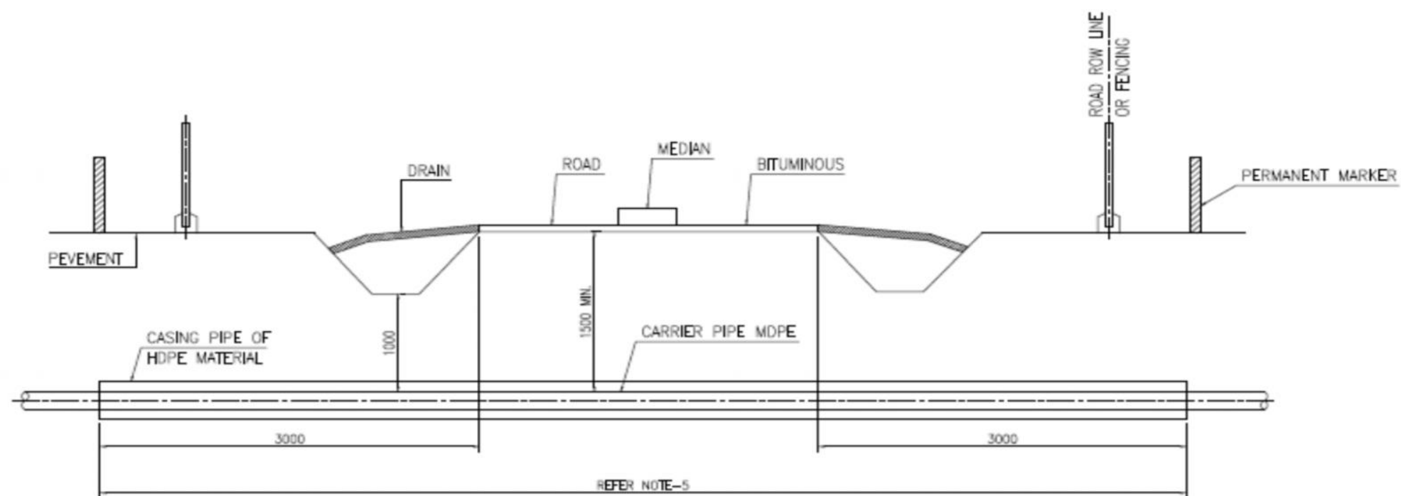
TYPICAL SECTION
