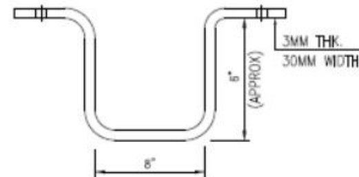
BRACKET FOR METERS (DOMESTIC)
