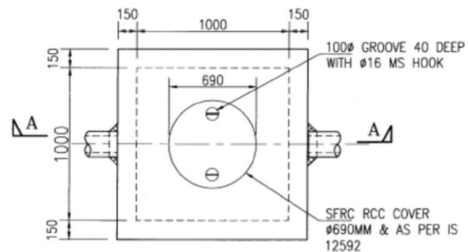
PLAN OF VALVE PIT VP-1
