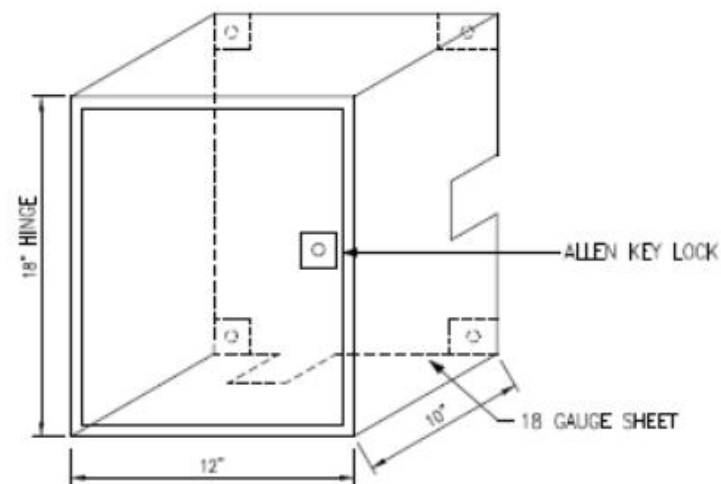
REGULATOR BOX
