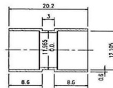
COUPLER
