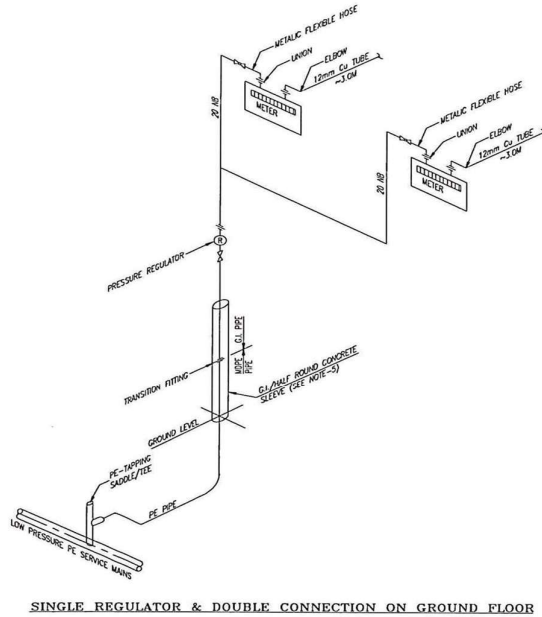
SINGLE REGULATOR & DOUBLE CONNECTION ON GROUND FLOOR
