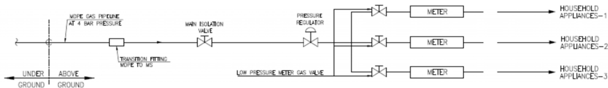
SCHEME OF NATURAL GAS SUPPLY TO DOMESTIC CONSUMERS
