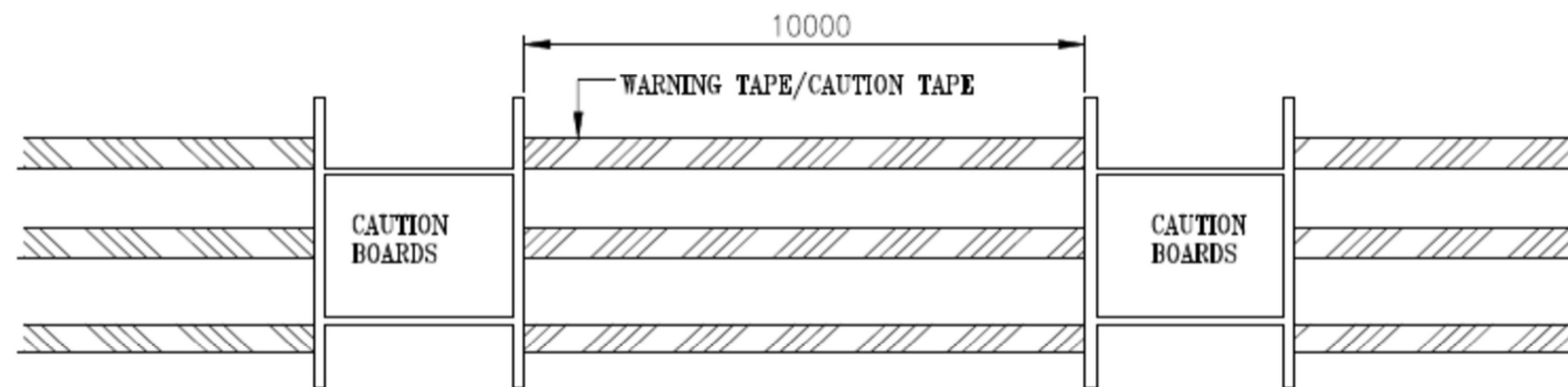
SCHEMATIC LAYOUT OF CAUTION BOARDS AND BARRICADDING
