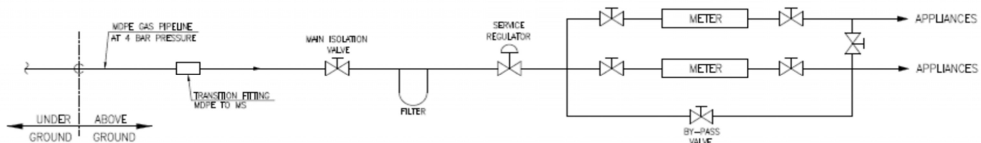
SCHEME OF NATURAL GAS SUPPLY TO LARGE COMMERCIAL CONSUMERS
