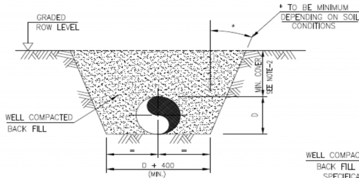
TRENCH IN NORMAL SOIL TYPICAL SECTION
