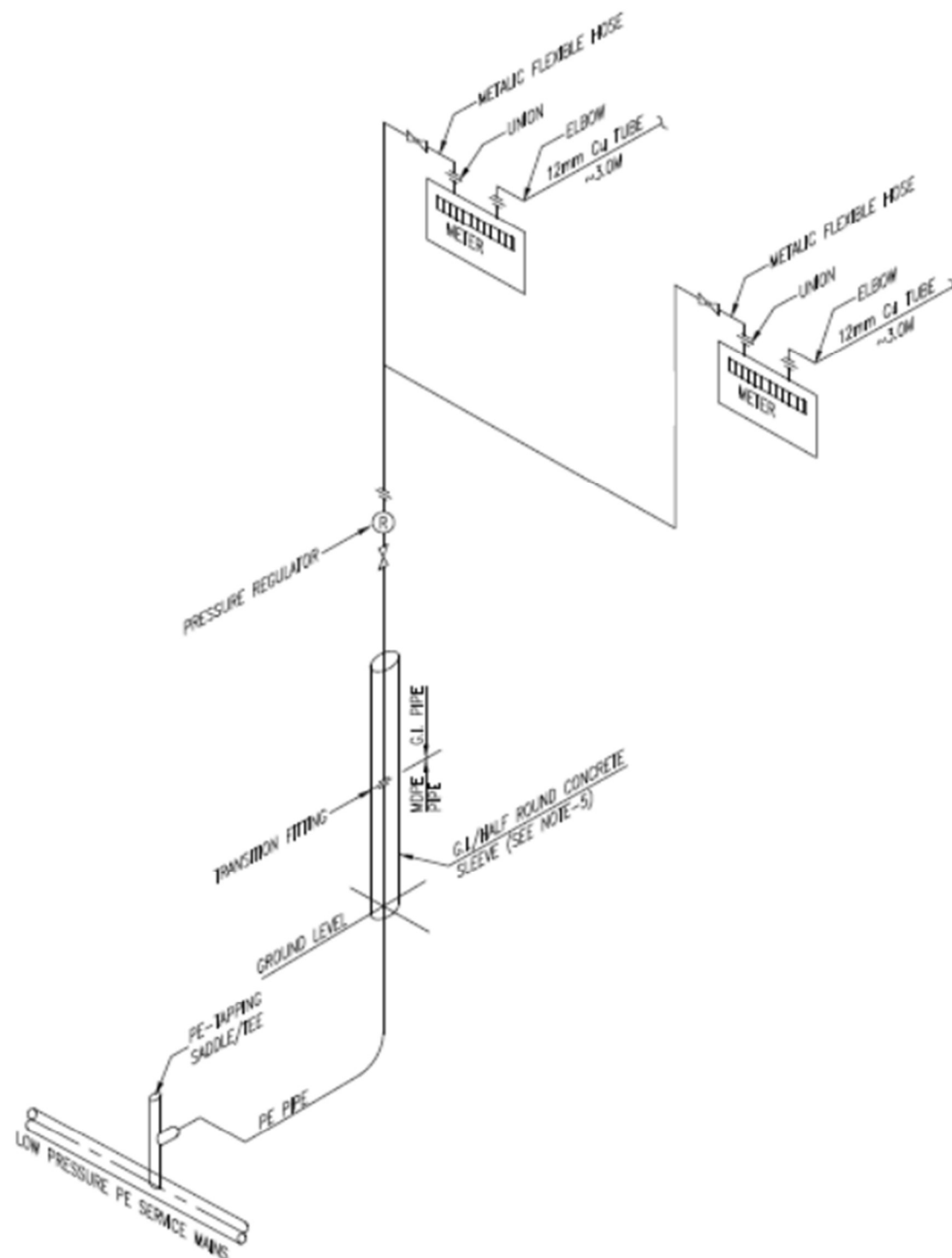
SINGLE REGULATOR & DOUBLE CONNECTION ON GROUND FLOOR
