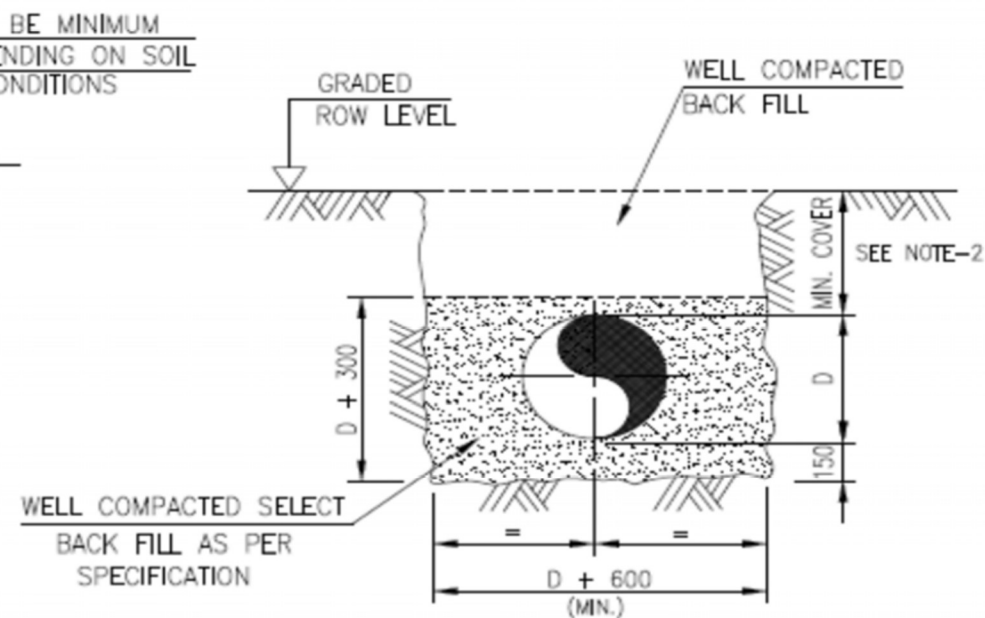
TRENCH IN CONSOLIDATED ROCK TYPICAL SECTION
