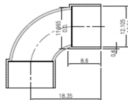
90° ELBOW
