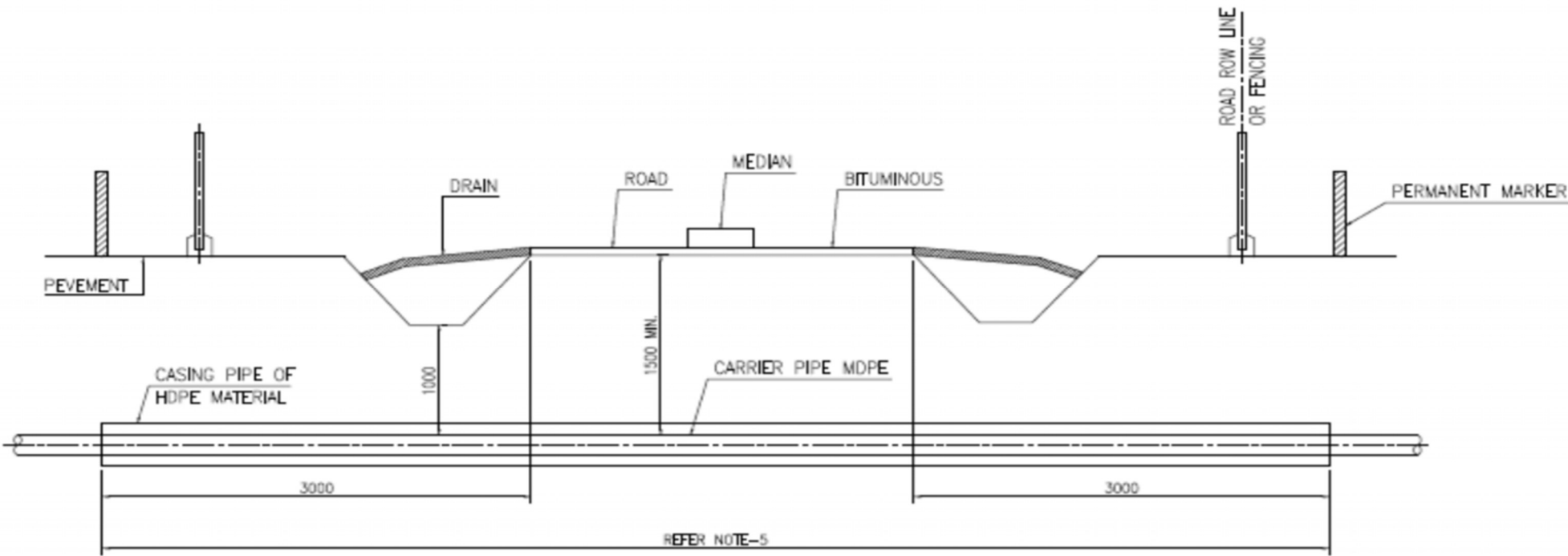
TYPICAL SECTION
