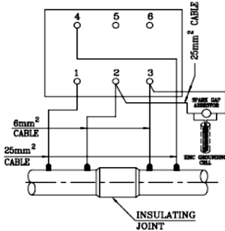
INSULATING JOINT (CONNECTION SCHEME-F)
