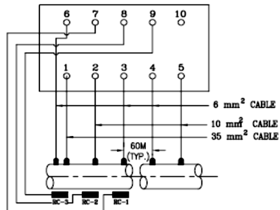
INTERMEDIATE STATION INPRESSED CURRENT DRAINAGE POINT (CONNECTION SCHEME-J)
