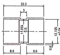
COUPLER
